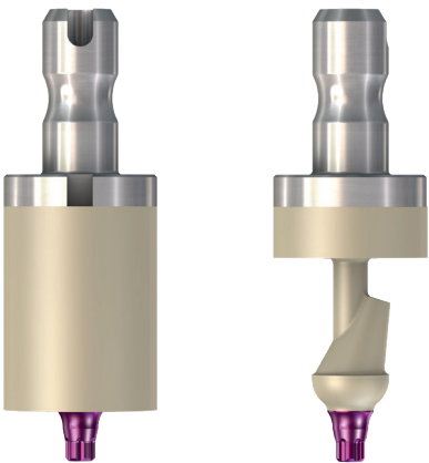
Prefabs made of BioHPP and grade 4 titanium KV with the original implant-abutment Connection
